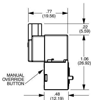
Straight/Out Coil with Normally Closed Valve
