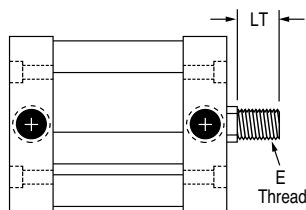
Male Rod Ends (Option CM or FM)
