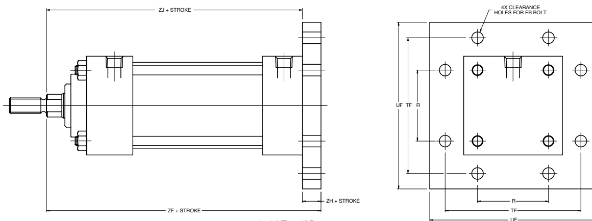
3-1/4" Thru 6" Bore
