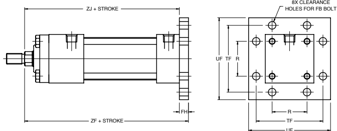
1-1/2" Thru 2-1/2" Bore
