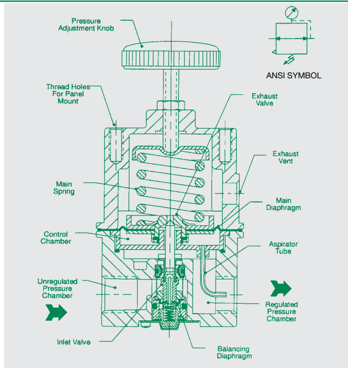
R880 Pictured Above (NOT R881)
