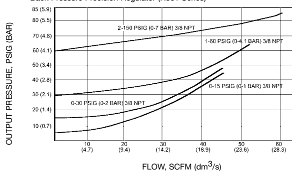
Back Pressure Precision Regulator (R881 Series)
